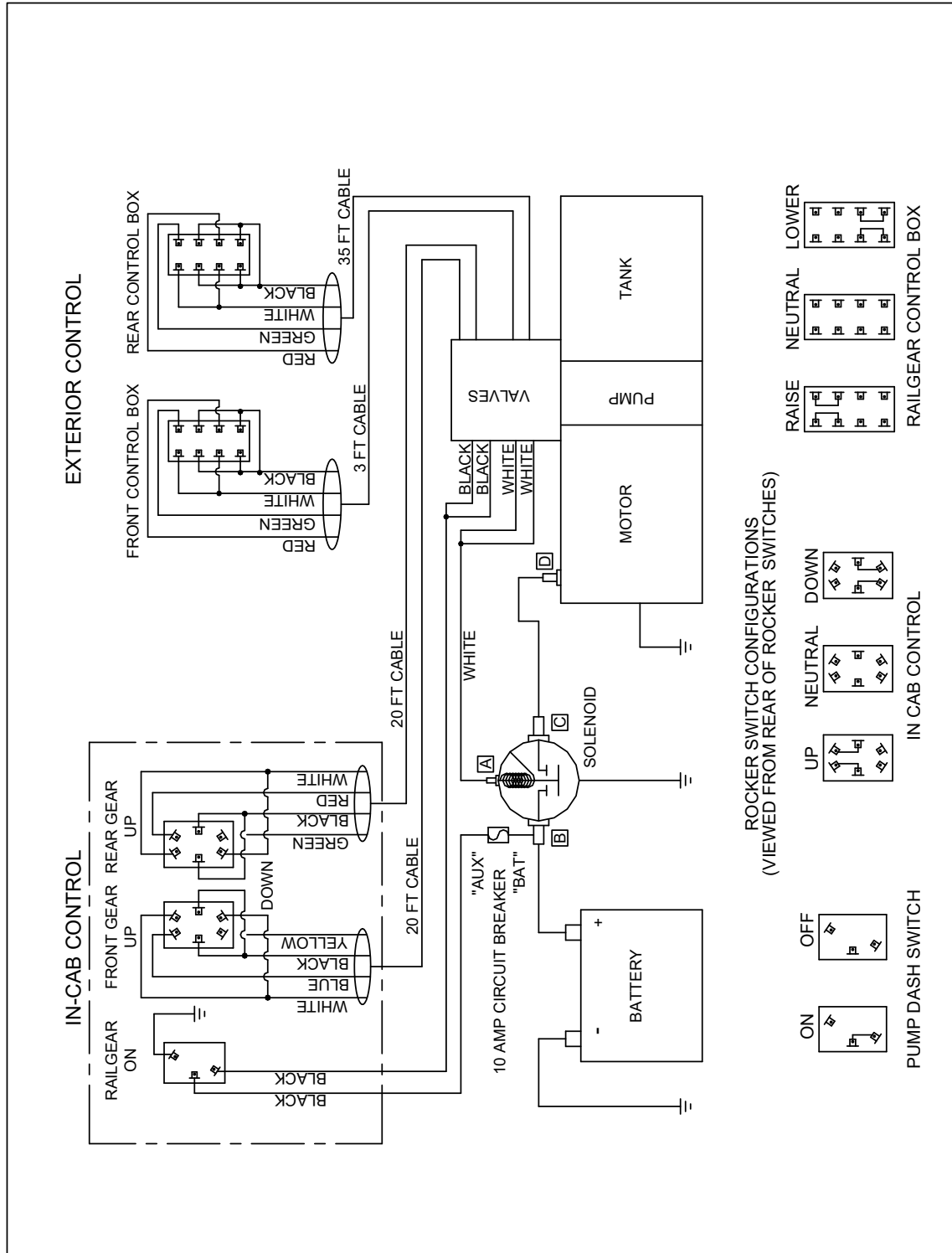
Figure 3: Electrical Schematic
