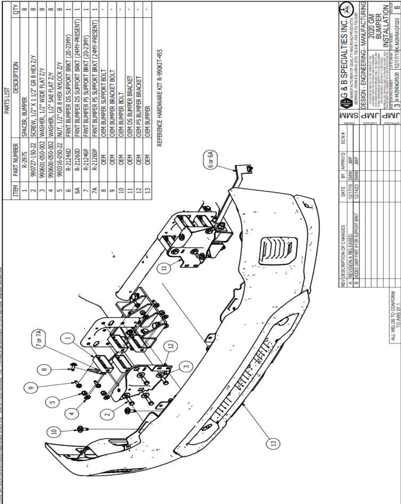
Figure 3 Bumper Installation
