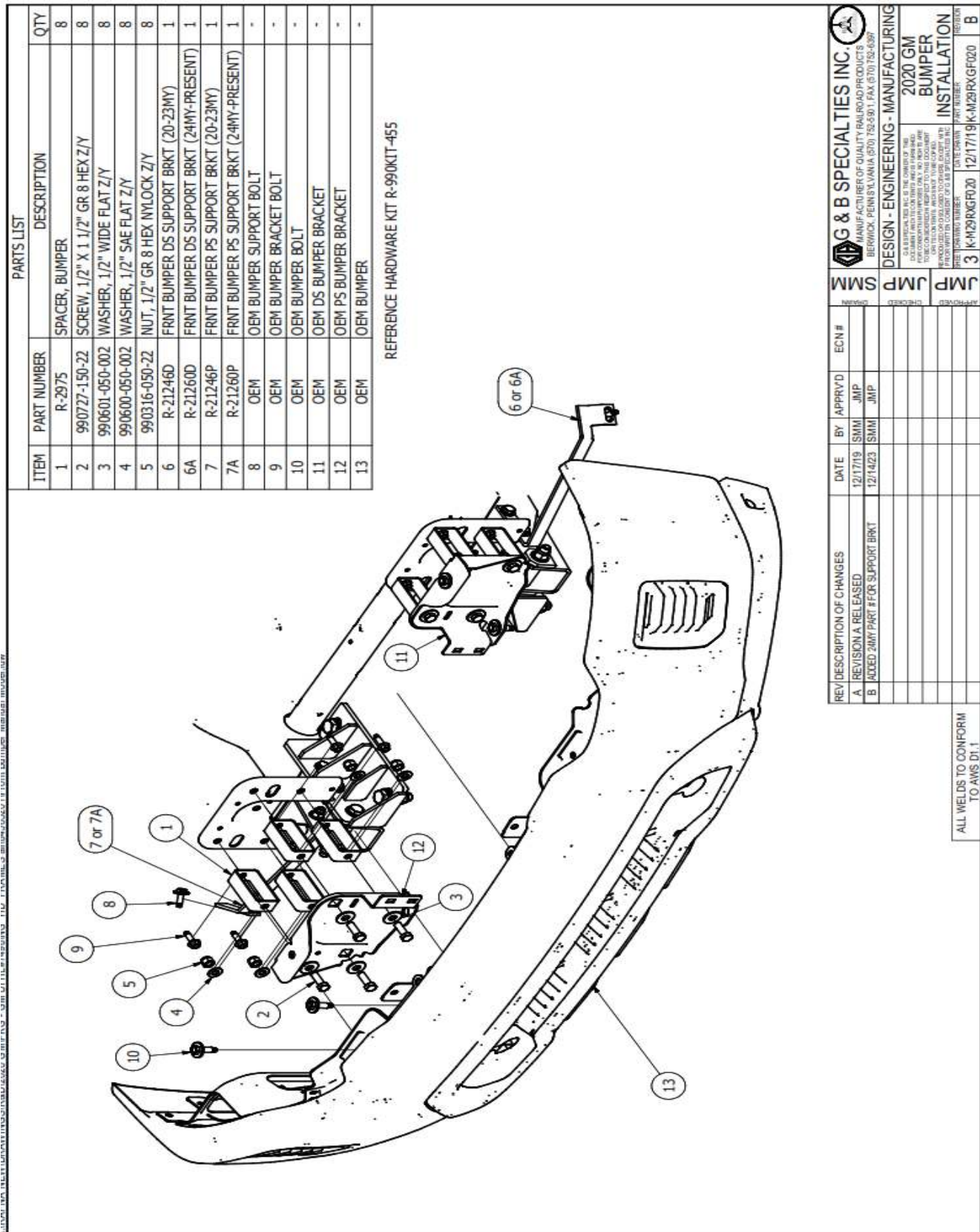
Figure 3 Bumper Installation
